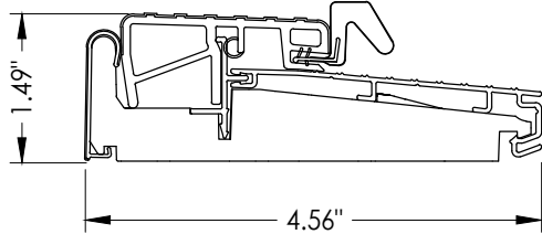
T9 OUTSWING THRESHOLD ZOB4565RDS
