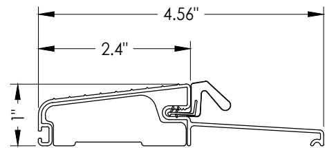
T10 OUTSWING THRESHOLD FOB4565
