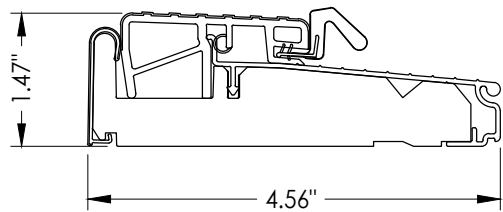
T8 OUTSWING THRESHOLD ZOB4565FN
