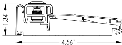
T6 INSWING ADJUSTABLE THRESHOLD ZAI4565RDS
