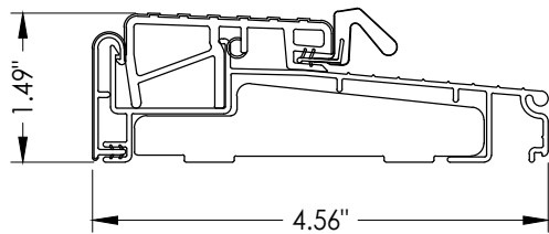
T7 OUTSWING THRESHOLD ZOBL4565
