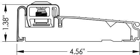
T5 INSWING ADJUSTABLE THRESHOLD ZAI4565FN
